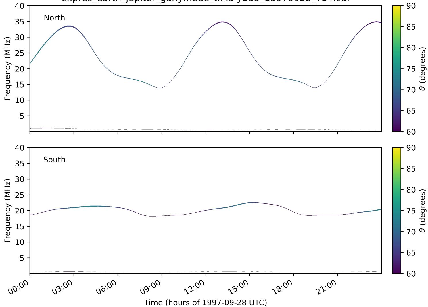
expres_earth_jupiter_ganymede_txka-y235_19970928_v14.cdf
