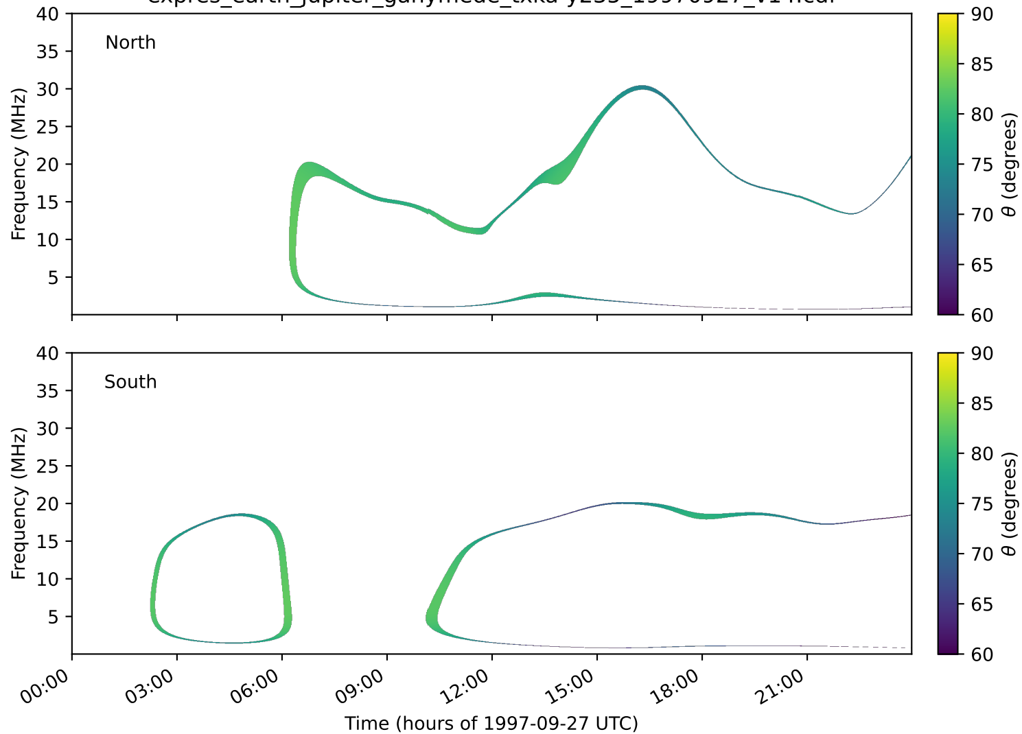
expres_earth_jupiter_ganymede_txka-y235_19970927_v14.cdf
