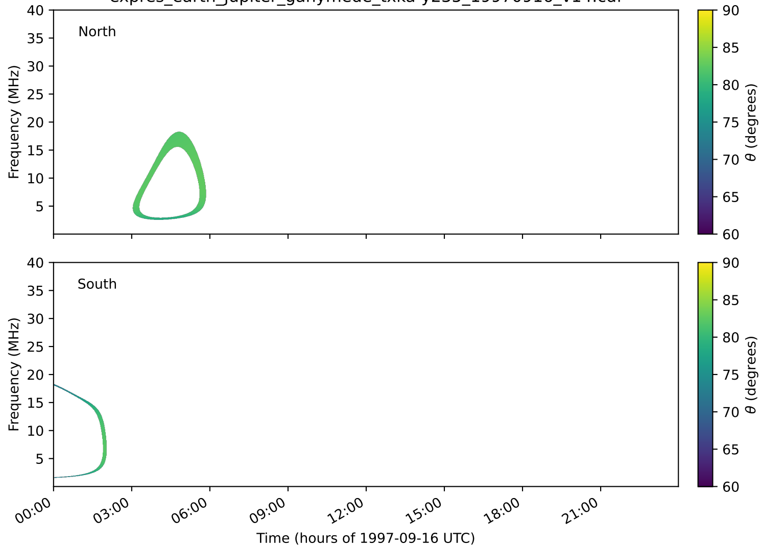
expres_earth_jupiter_ganymede_txka-y235_19970916_v14.cdf
