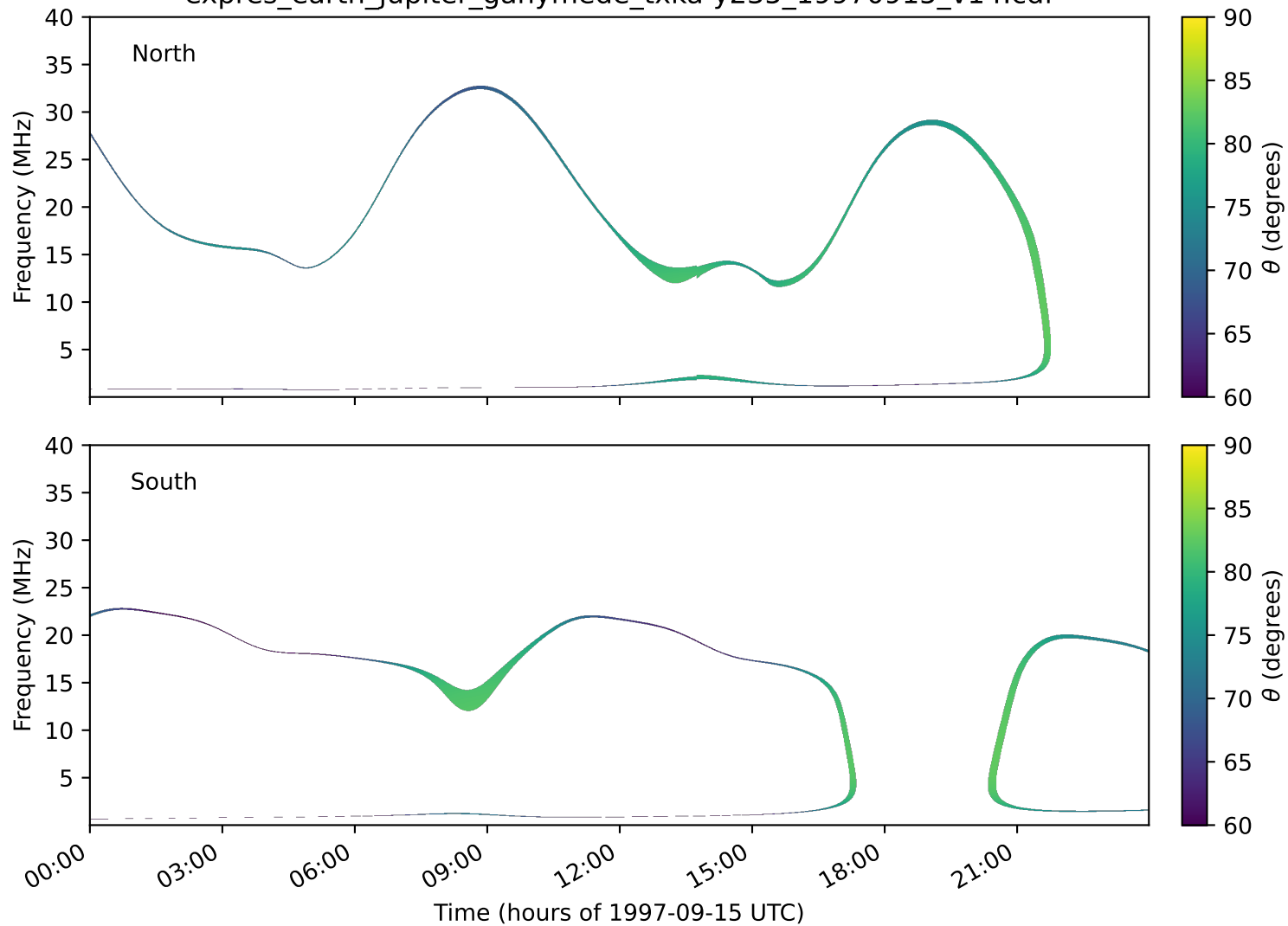
expres_earth_jupiter_ganymede_txka-y235_19970915_v14.cdf
