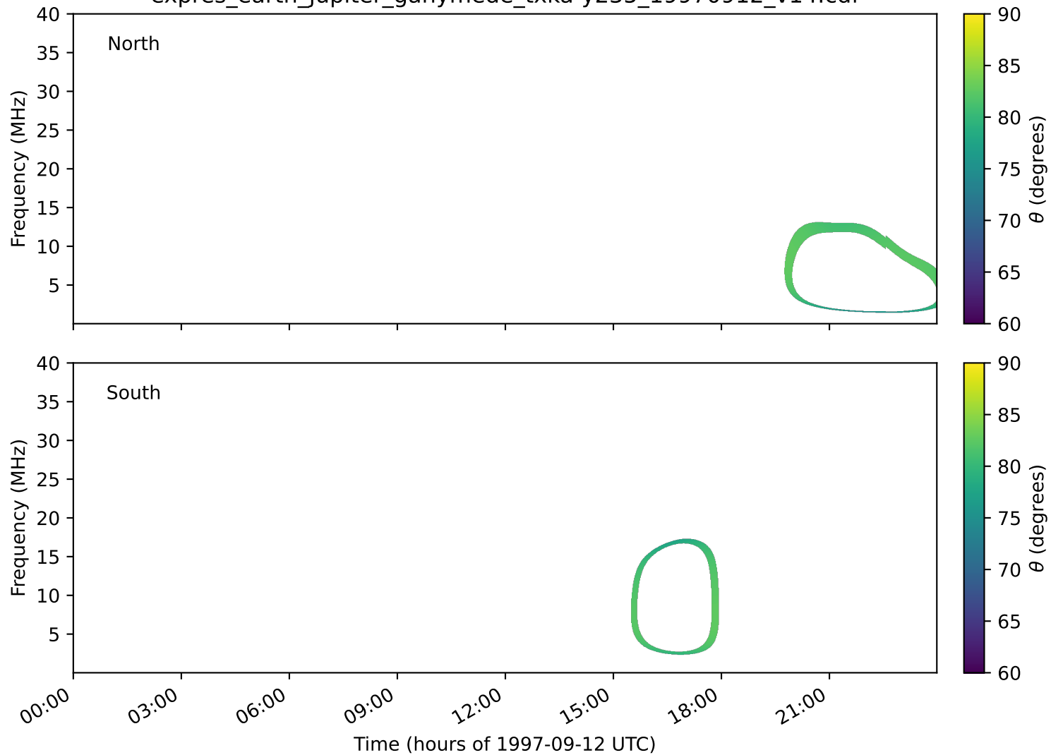
expres_earth_jupiter_ganymede_txka-y235_19970912_v14.cdf
