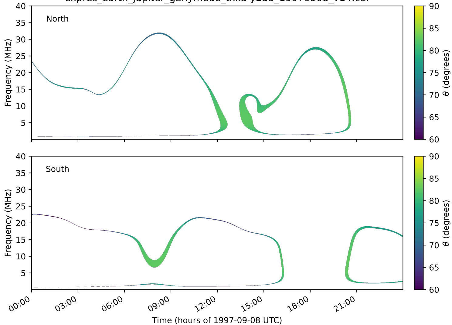
expres_earth_jupiter_ganymede_txka-y235_19970908_v14.cdf
