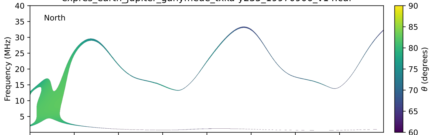
expres_earth_jupiter_ganymede_txka-y235_19970906_v14.cdf
