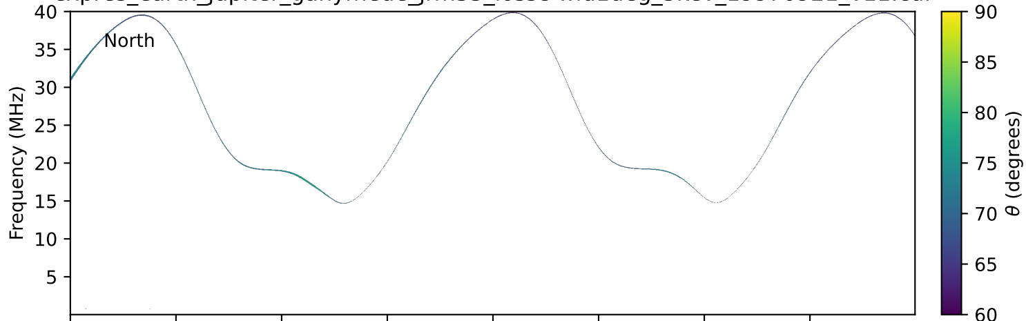
expres_earth_jupiter_ganymede_jrm33_lossc-wid1deg_3kev_19970921_v11.cdf
