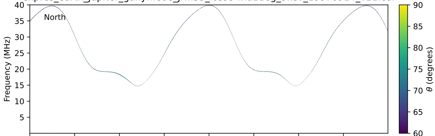
expres_earth_jupiter_ganymede_jrm33_lossc-wid1deg_3kev_19970914_v11.cdf
