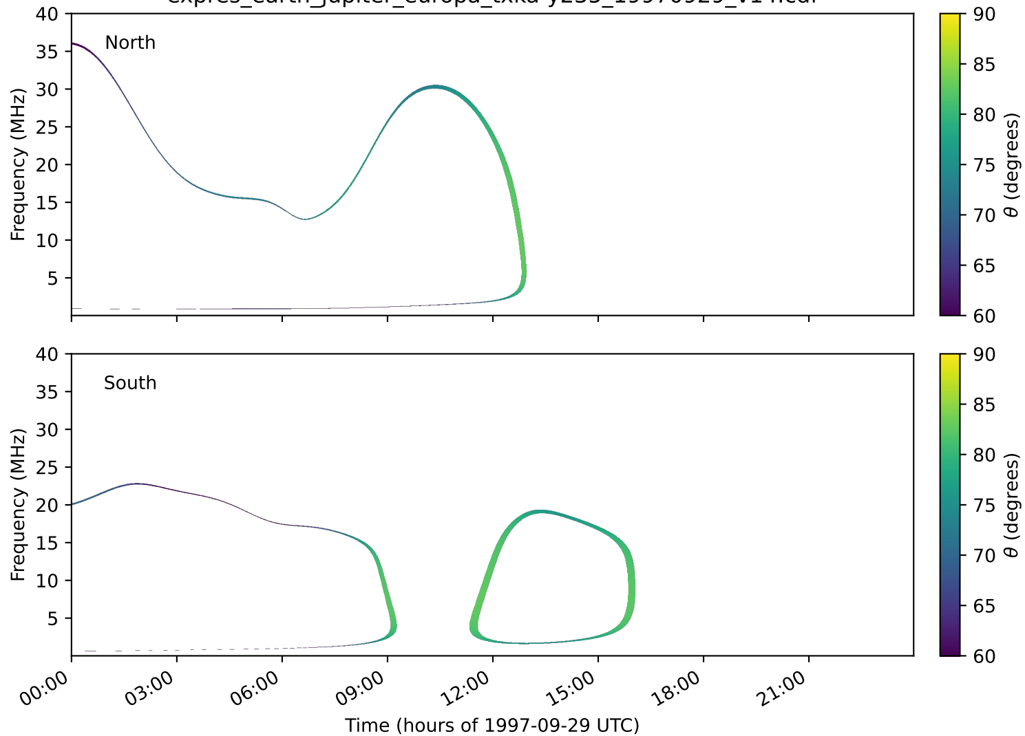
expres_earth_jupiter_europa_txka-y235_19970929_v14.cdf
