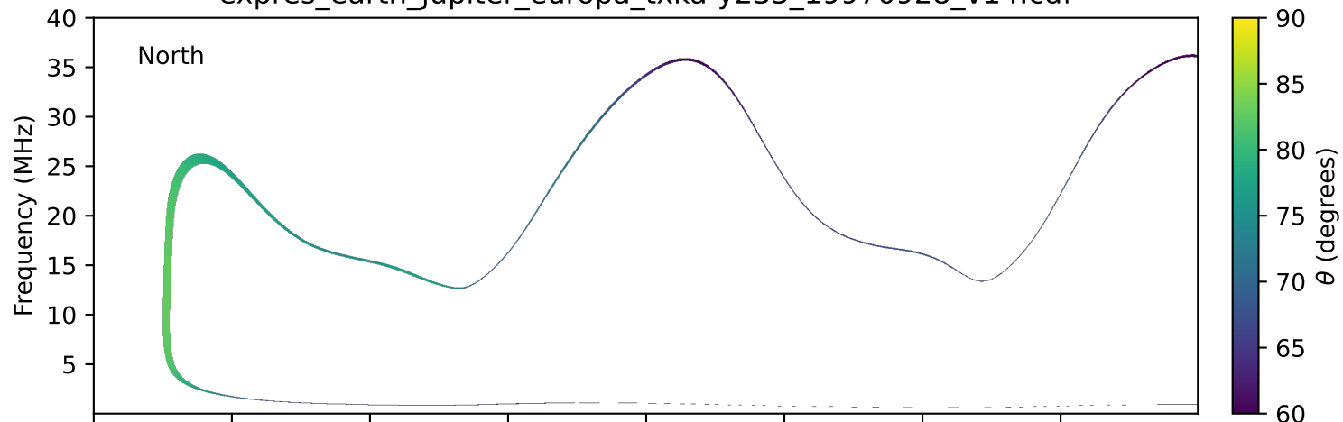
expres_earth_jupiter_europa_txka-y235_19970928_v14.cdf
