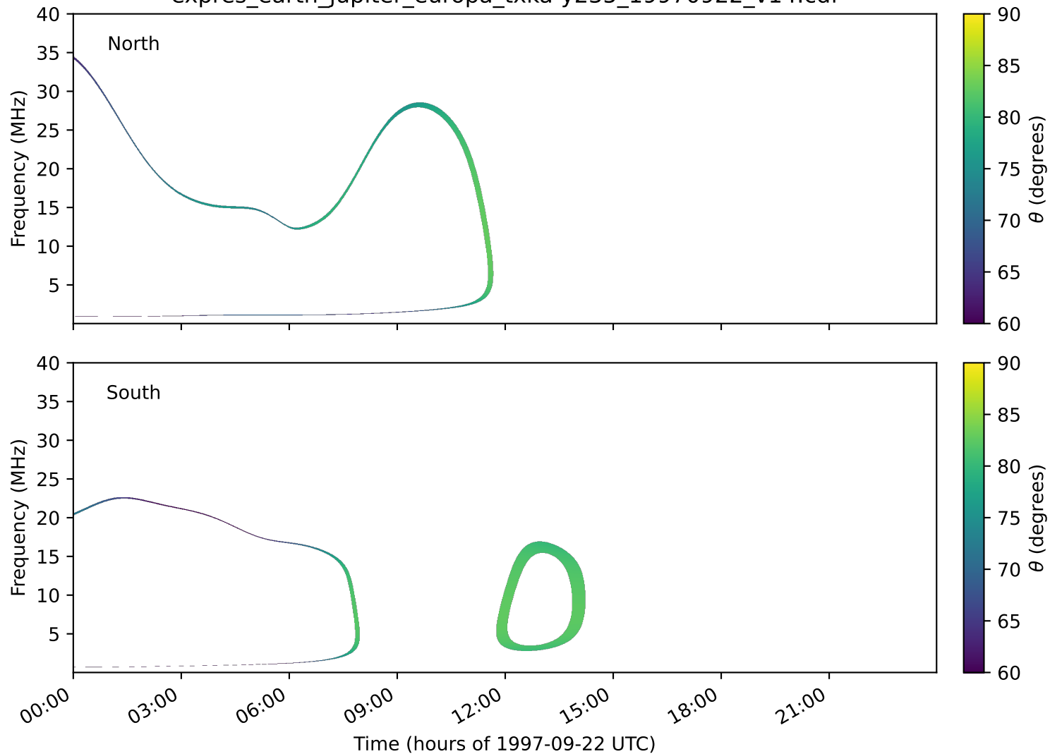
expres_earth_jupiter_europa_txka-y235_19970922_v14.cdf
