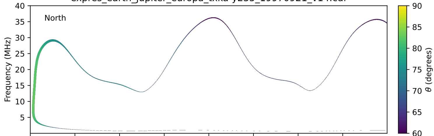
expres_earth_jupiter_europa_txka-y235_19970921_v14.cdf
