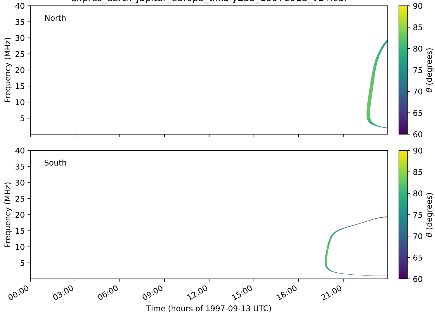
expres_earth_jupiter_europa_txka-y235_19970913_v14.cdf
