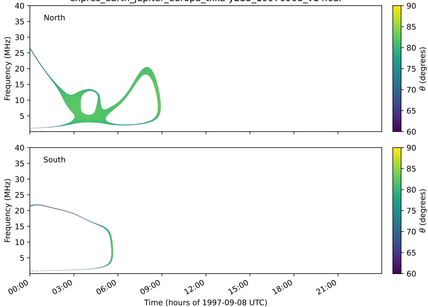
expres_earth_jupiter_europa_txka-y235_19970908_v14.cdf
