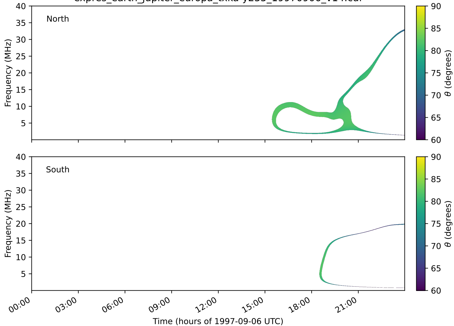
expres_earth_jupiter_europa_txka-y235_19970906_v14.cdf
