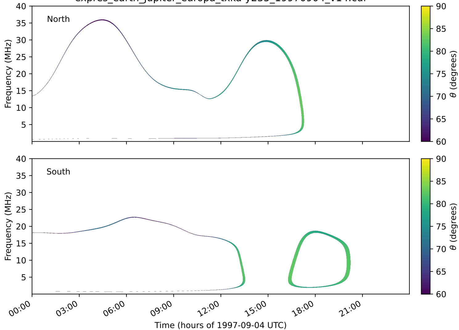
expres_earth_jupiter_europa_txka-y235_19970904_v14.cdf
