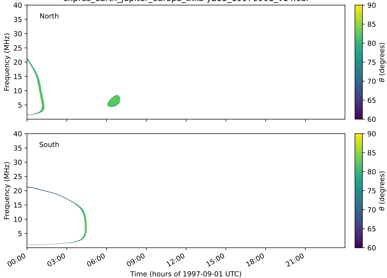
expres_earth_jupiter_europa_txka-y235_19970901_v14.cdf
