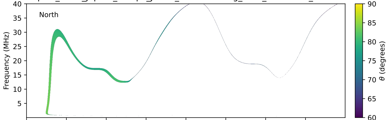
expres_earth_jupiter_europa_jrm33_lossc-wid1deg_3kev_19970928_v11.cdf
