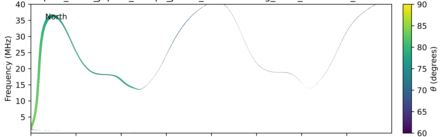
expres_earth_jupiter_europa_jrm33_lossc-wid1deg_3kev_19970921_v11.cdf
