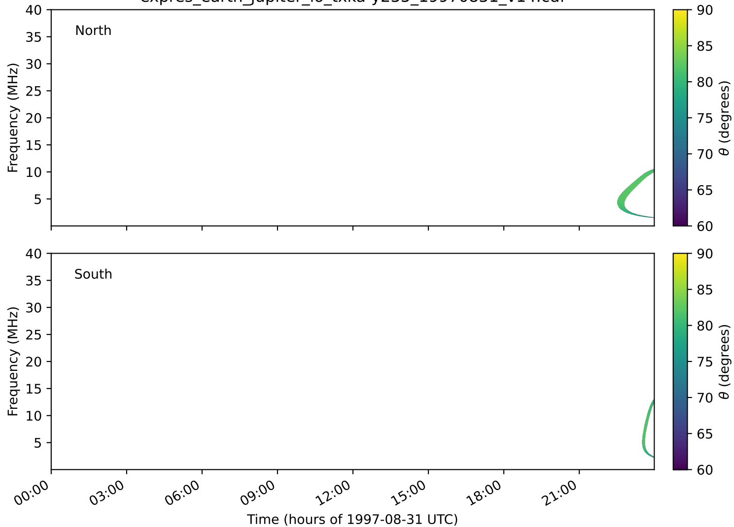
expres_earth_jupiter_io_txka-y235_19970831_v14.cdf
