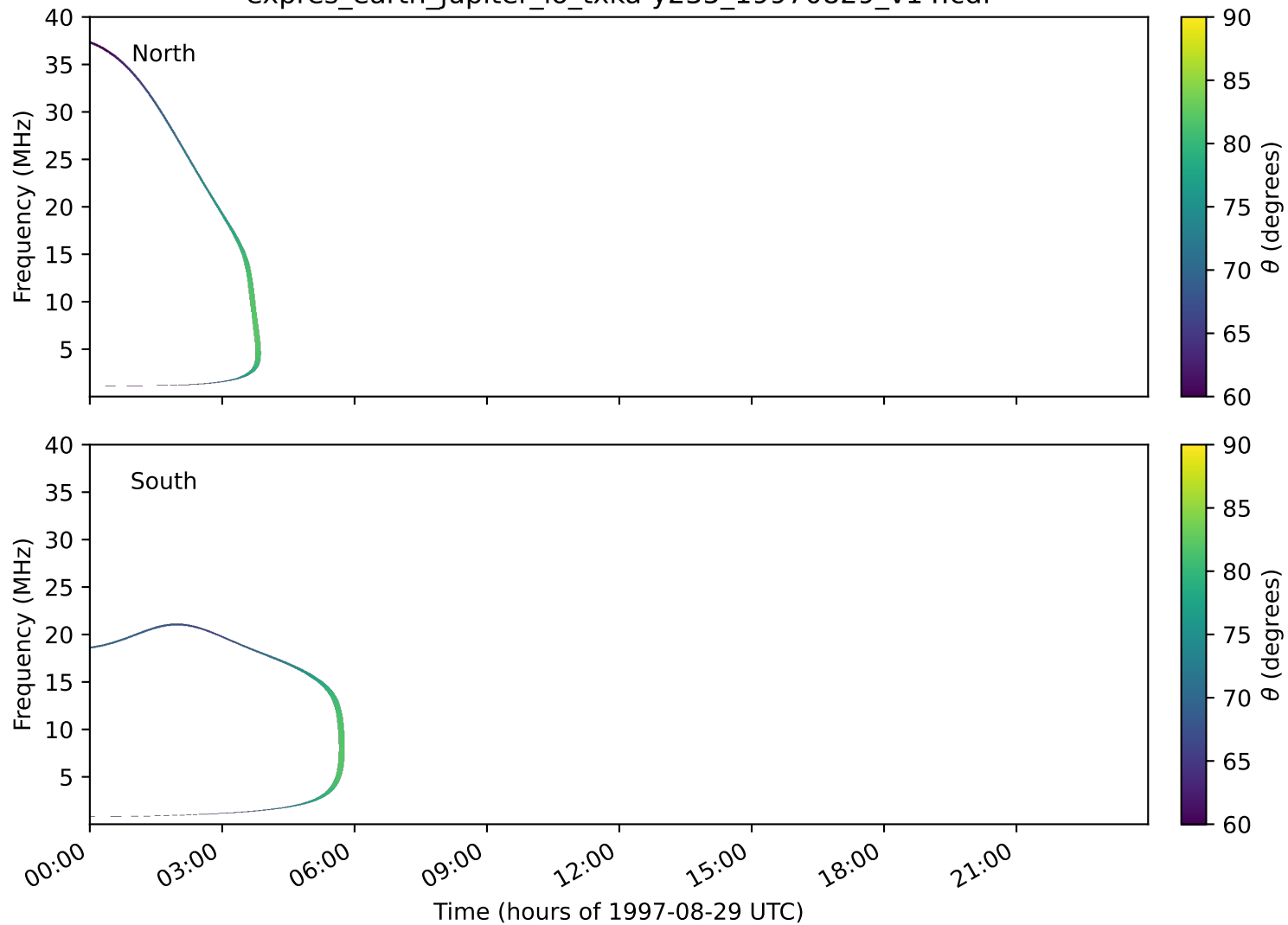
expres_earth_jupiter_io_txka-y235_19970829_v14.cdf
