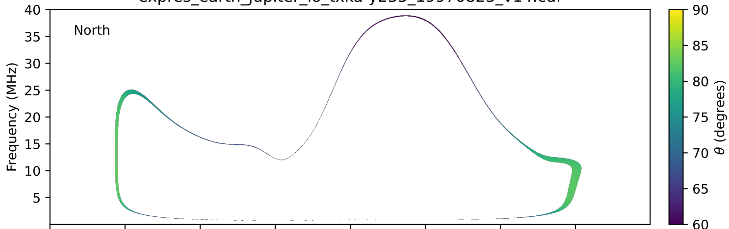
expres_earth_jupiter_io_txka-y235_19970823_v14.cdf
