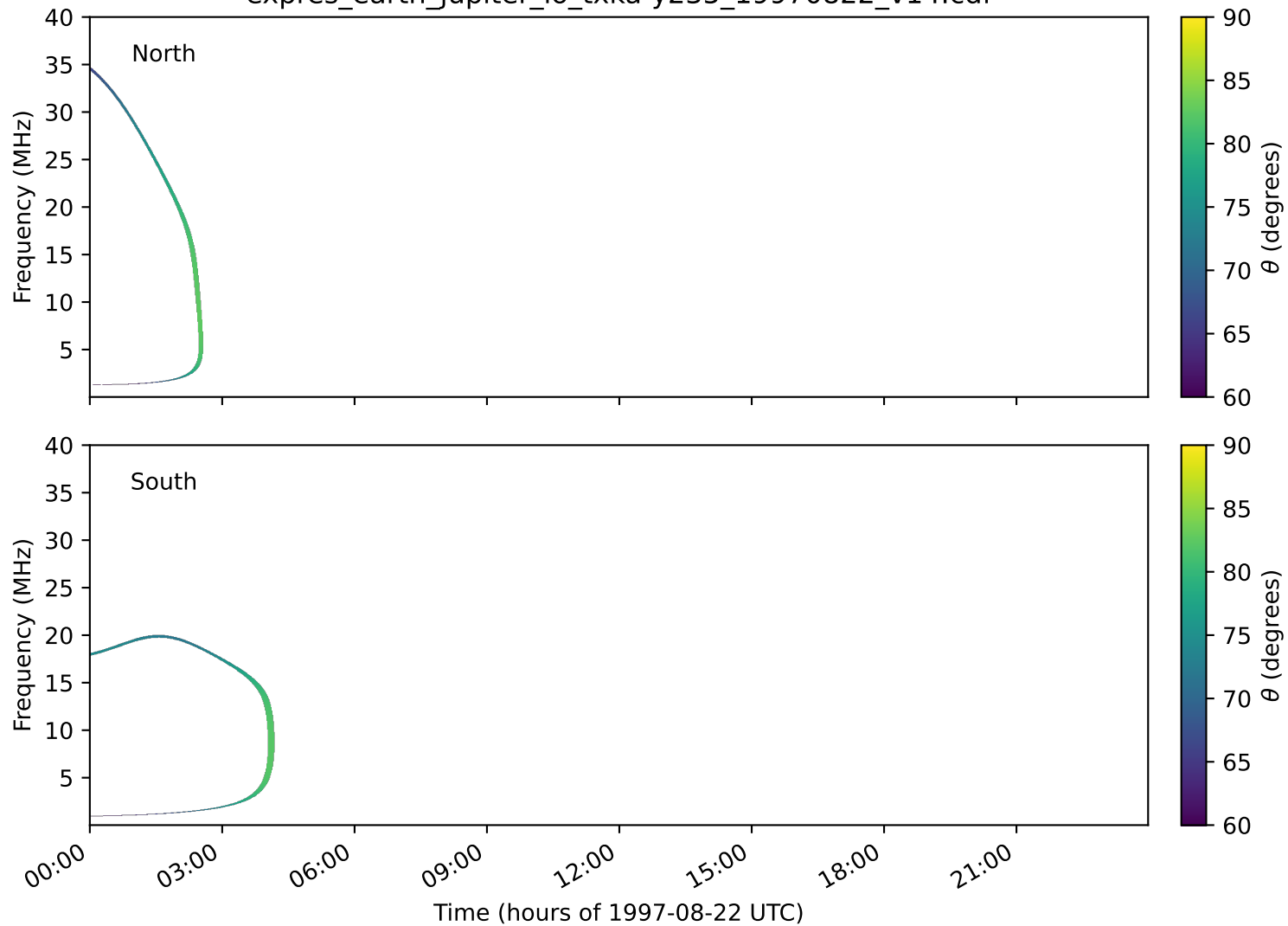
expres_earth_jupiter_io_txka-y235_19970822_v14.cdf
