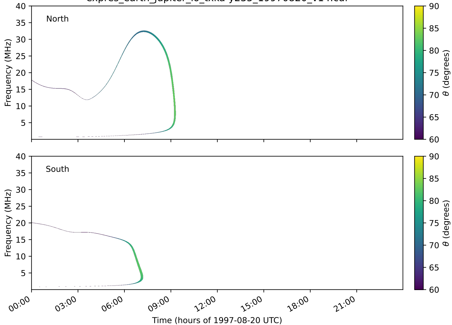
expres_earth_jupiter_io_txka-y235_19970820_v14.cdf
