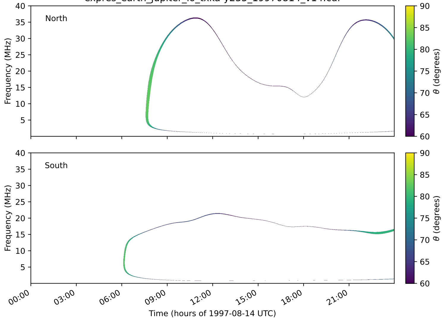
expres_earth_jupiter_io_txka-y235_19970814_v14.cdf
