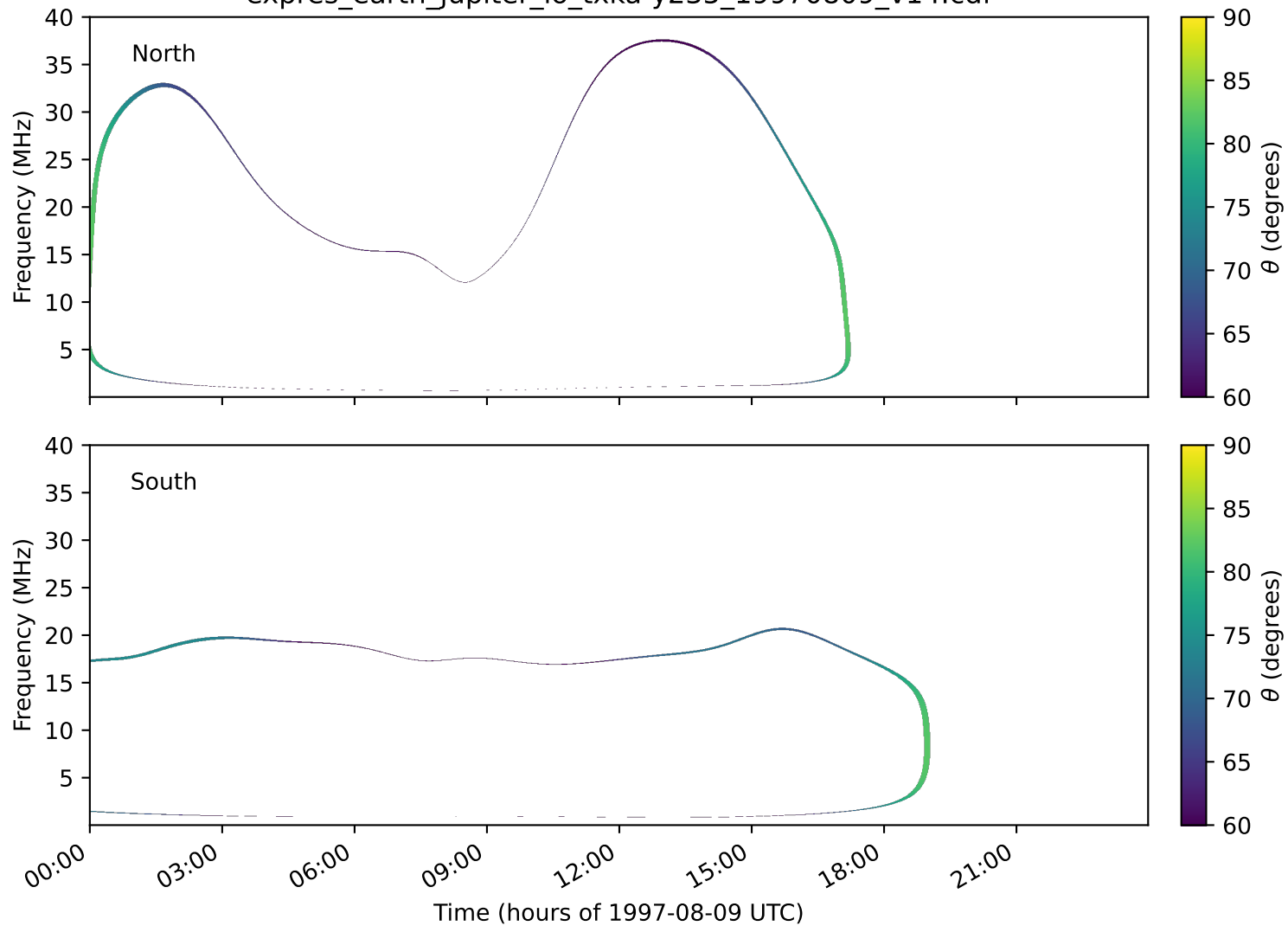
expres_earth_jupiter_io_txka-y235_19970809_v14.cdf
