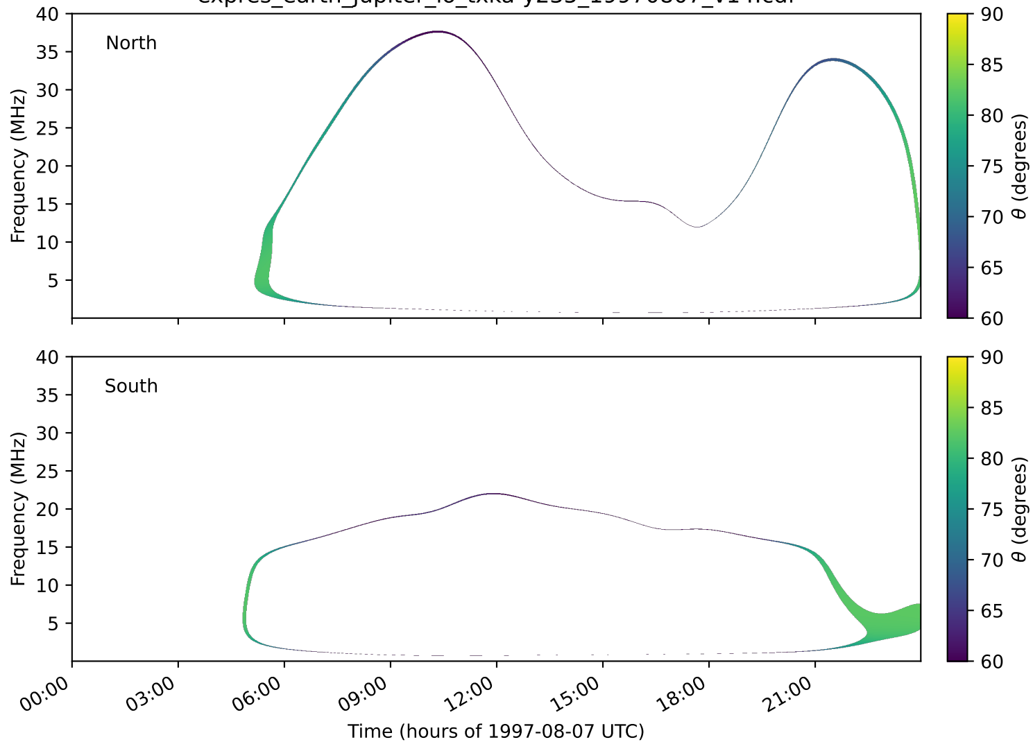
expres_earth_jupiter_io_txka-y235_19970807_v14.cdf
