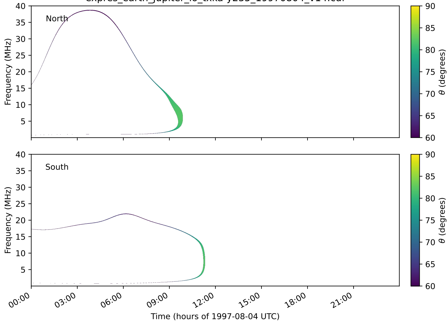
expres_earth_jupiter_io_txka-y235_19970804_v14.cdf
