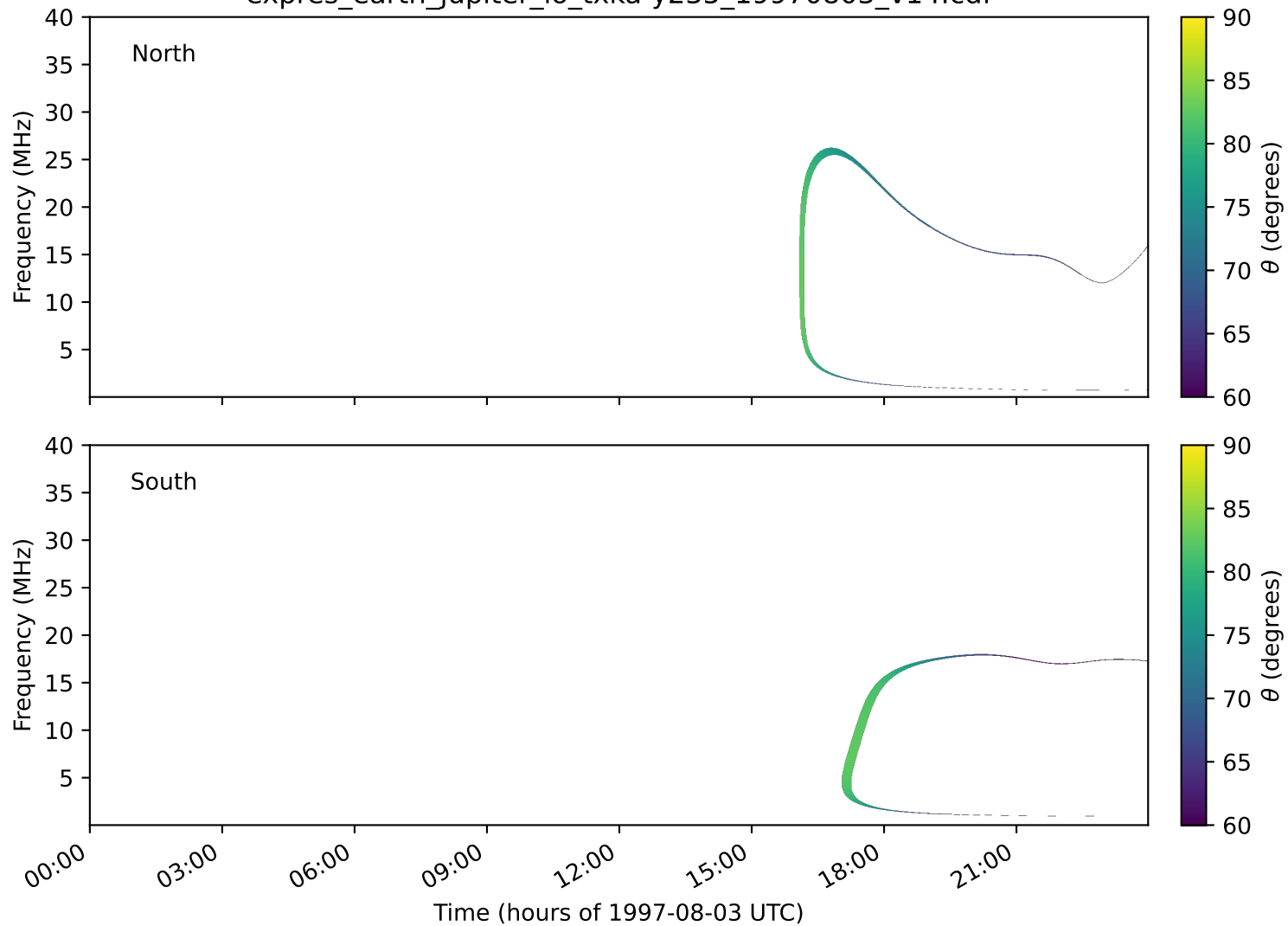
expres_earth_jupiter_io_txka-y235_19970803_v14.cdf
