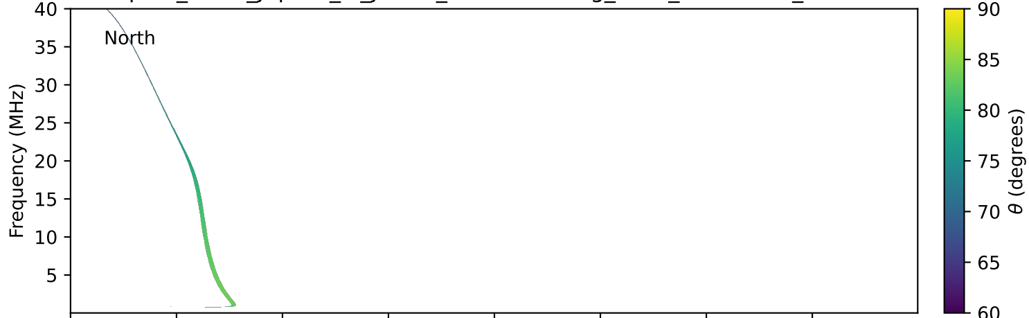
expres_earth_jupiter_io_jrm33_lossc-wid1deg_3kev_19970829_v11.cdf
