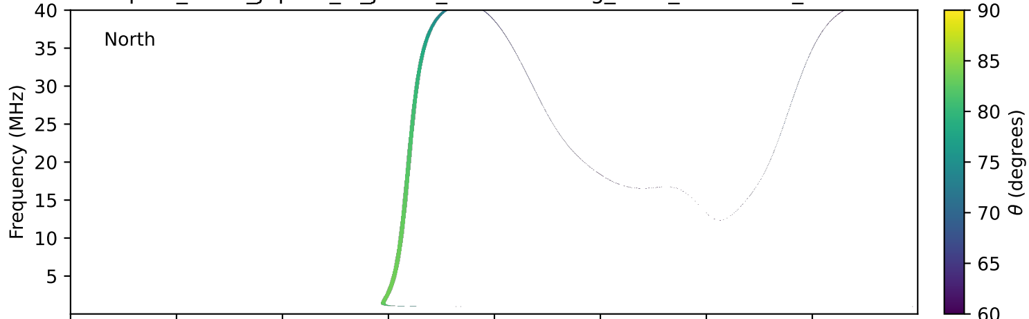
expres_earth_jupiter_io_jrm33_lossc-wid1deg_3kev_19970821_v11.cdf
