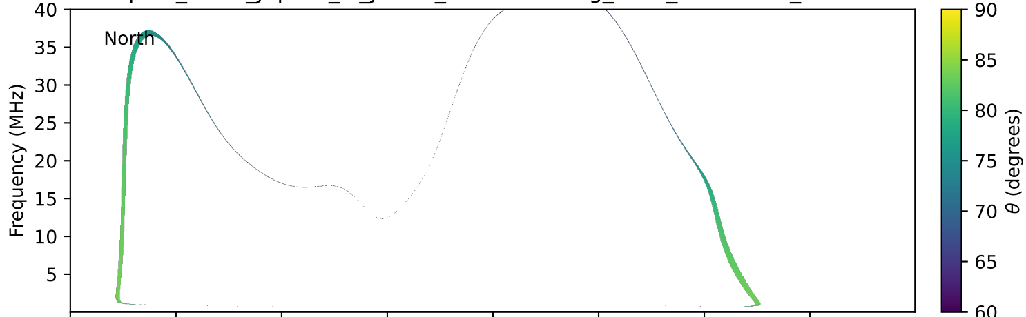
expres_earth_jupiter_io_jrm33_lossc-wid1deg_3kev_19970816_v11.cdf
