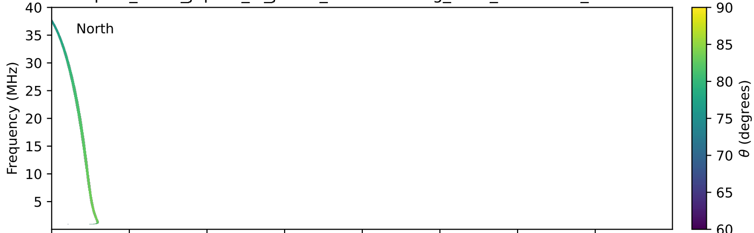
expres_earth_jupiter_io_jrm33_lossc-wid1deg_3kev_19970815_v11.cdf
