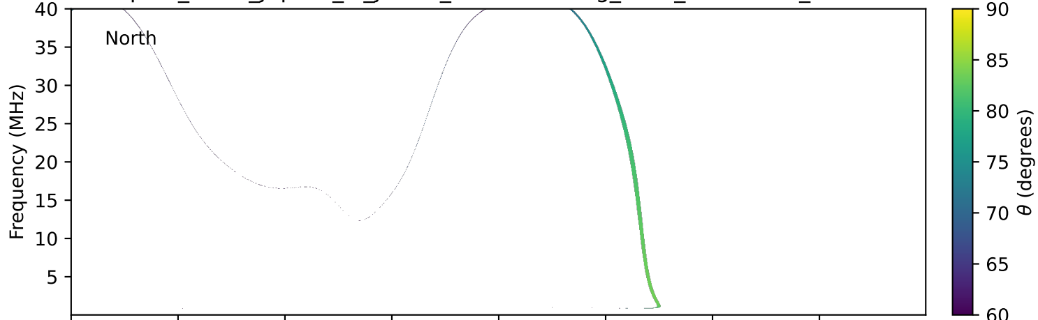
expres_earth_jupiter_io_jrm33_lossc-wid1deg_3kev_19970802_v11.cdf
