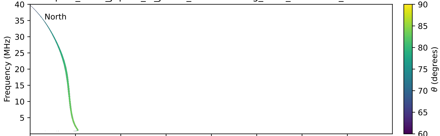
expres_earth_jupiter_io_jrm09_lossc-wid1deg_3kev_19970822_v11.cdf
