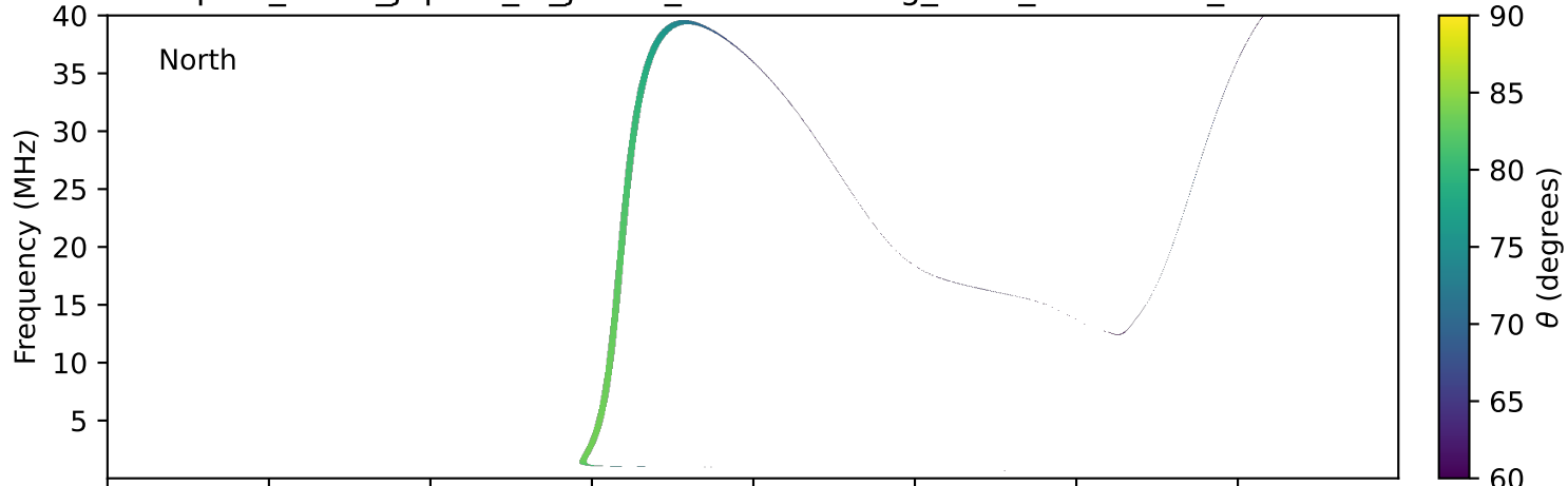
expres_earth_jupiter_io_jrm09_lossc-wid1deg_3kev_19970821_v11.cdf
