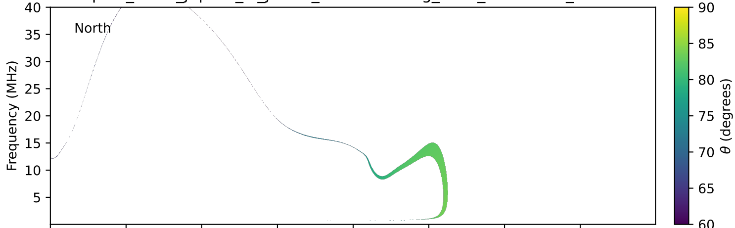
expres_earth_jupiter_io_jrm09_lossc-wid1deg_3kev_19970818_v11.cdf
