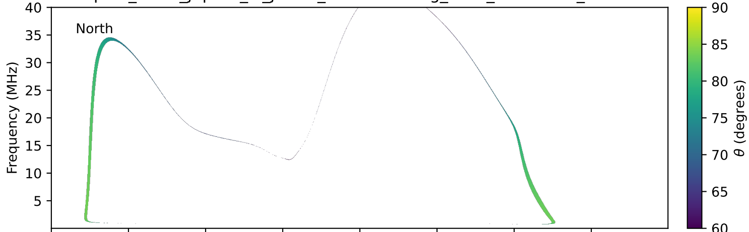
expres_earth_jupiter_io_jrm09_lossc-wid1deg_3kev_19970816_v11.cdf
