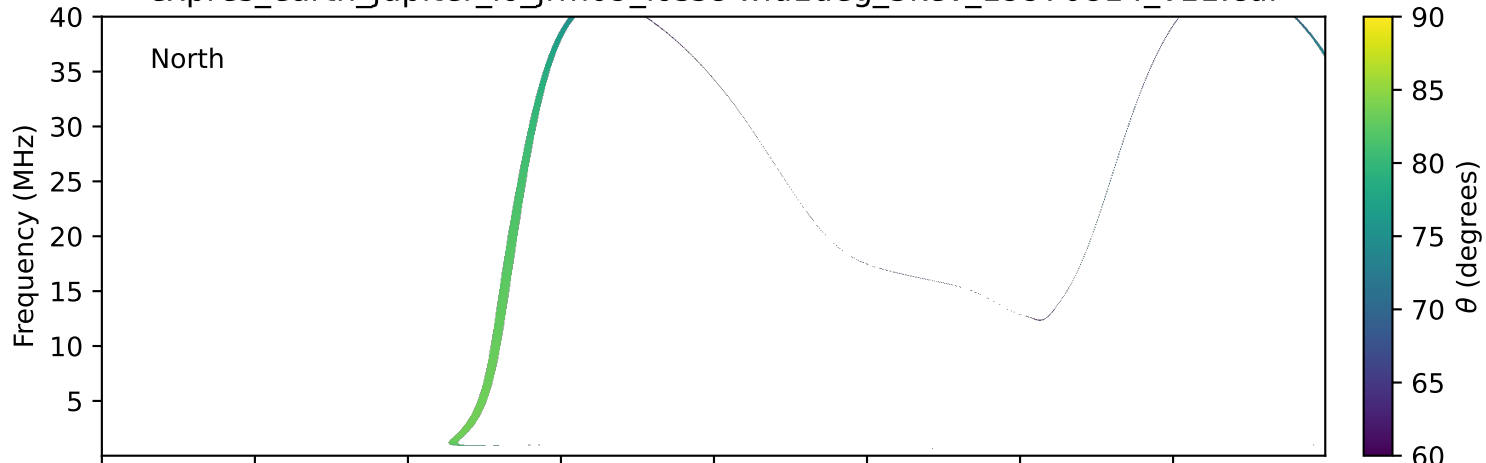
expres_earth_jupiter_io_jrm09_lossc-wid1deg_3kev_19970814_v11.cdf
