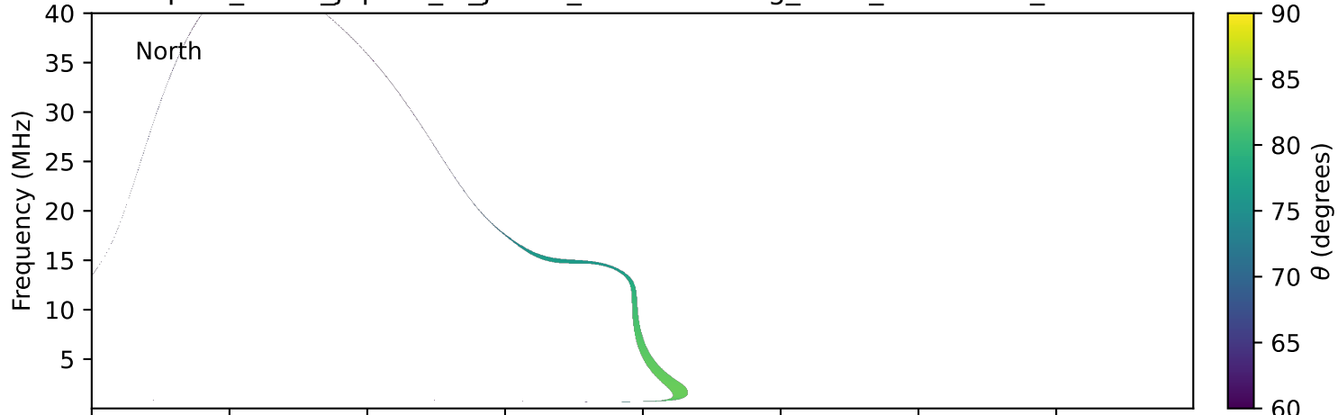
expres_earth_jupiter_io_jrm09_lossc-wid1deg_3kev_19970811_v11.cdf
