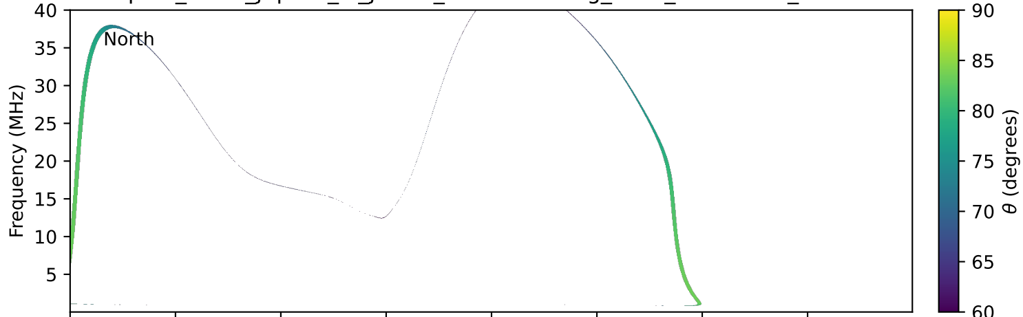
expres_earth_jupiter_io_jrm09_lossc-wid1deg_3kev_19970809_v11.cdf
