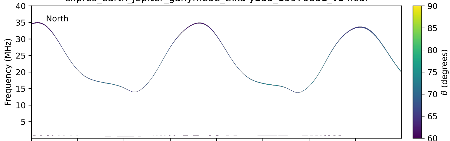
expres_earth_jupiter_ganymede_txka-y235_19970831_v14.cdf
