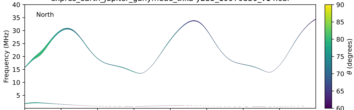
expres_earth_jupiter_ganymede_txka-y235_19970830_v14.cdf
