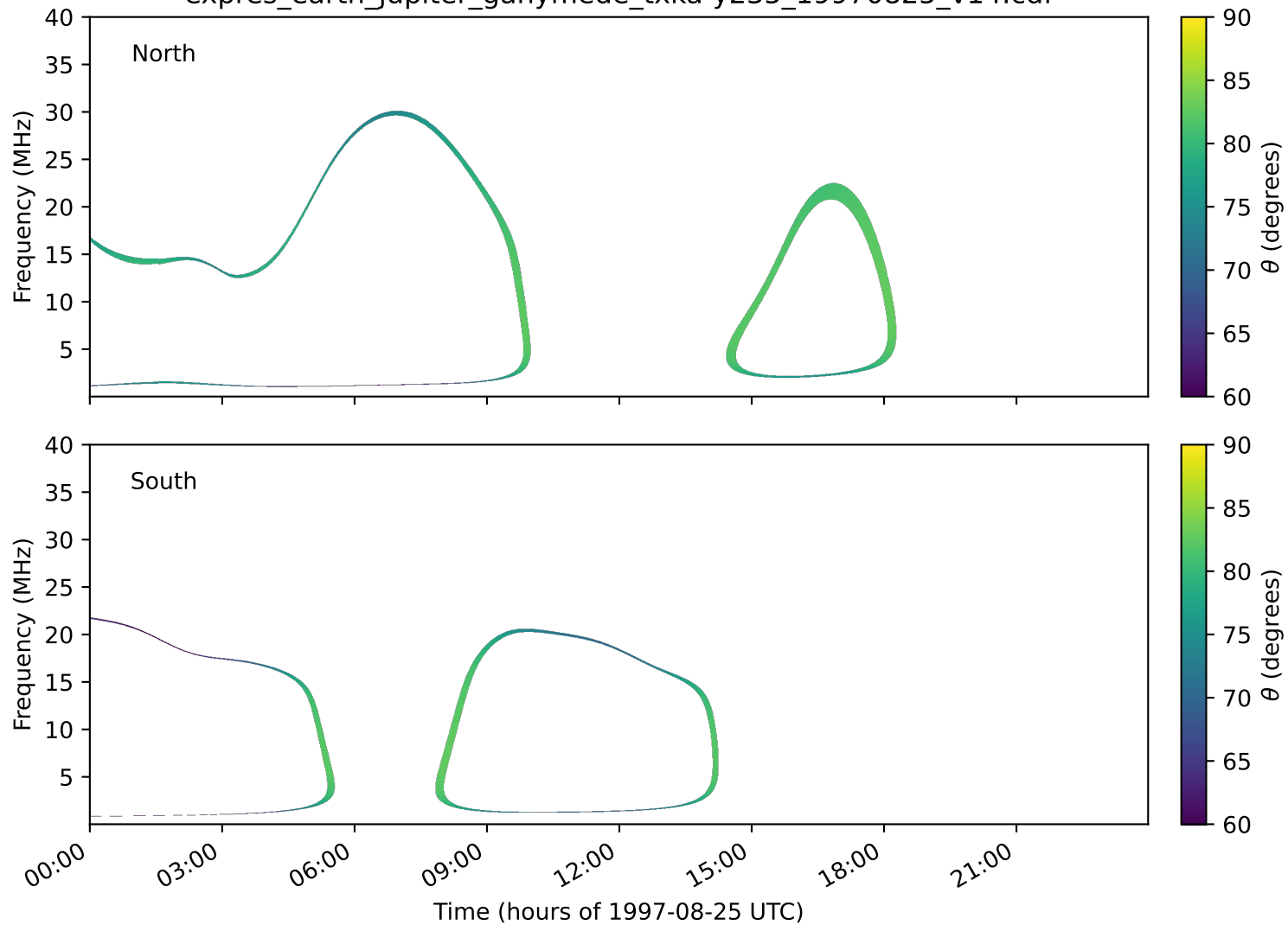
expres_earth_jupiter_ganymede_txka-y235_19970825_v14.cdf
