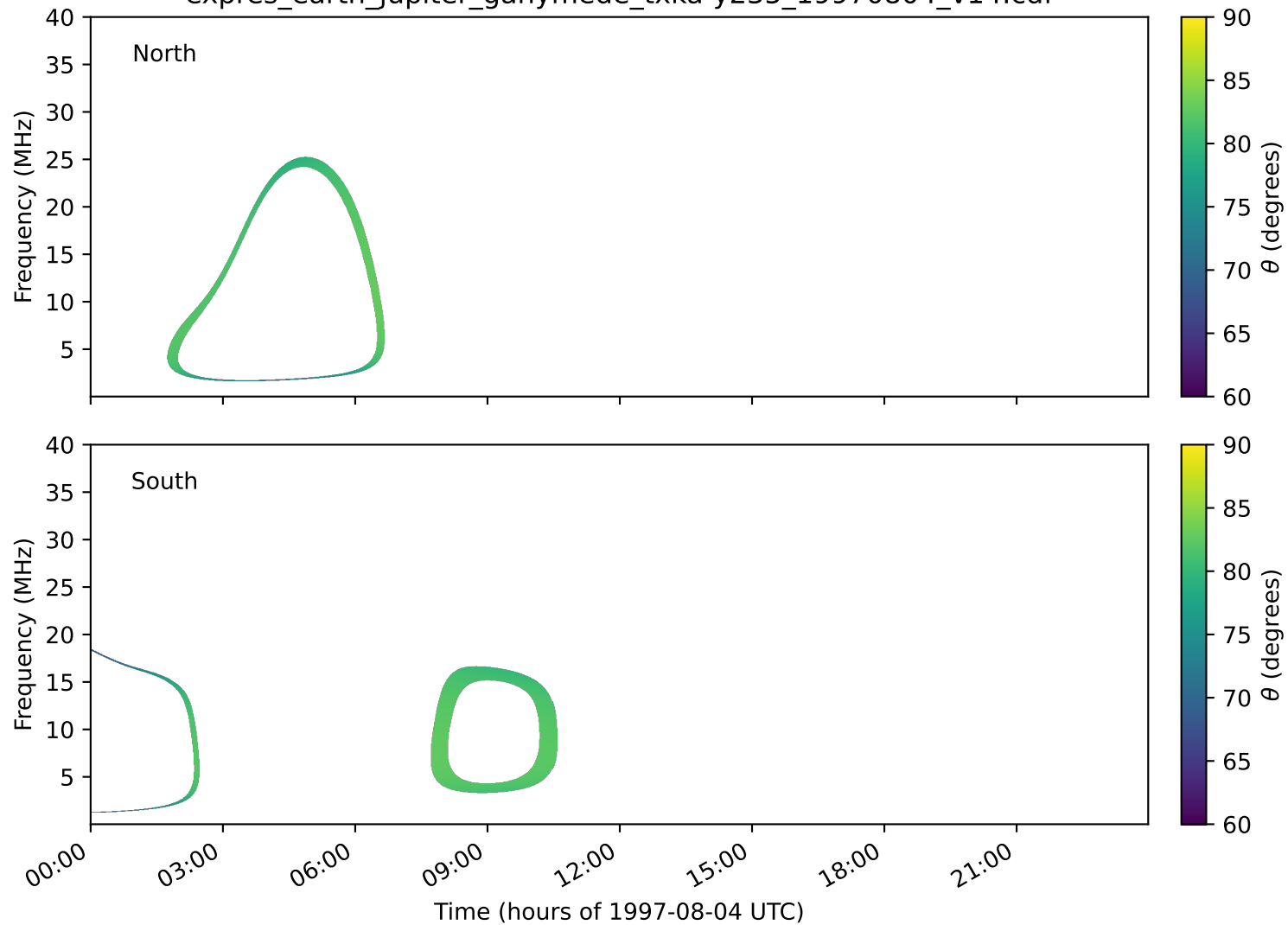
expres_earth_jupiter_ganymede_txka-y235_19970804_v14.cdf
