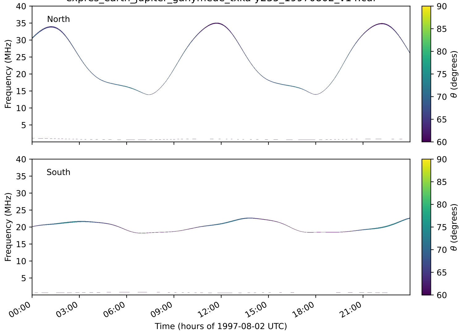
expres_earth_jupiter_ganymede_txka-y235_19970802_v14.cdf
