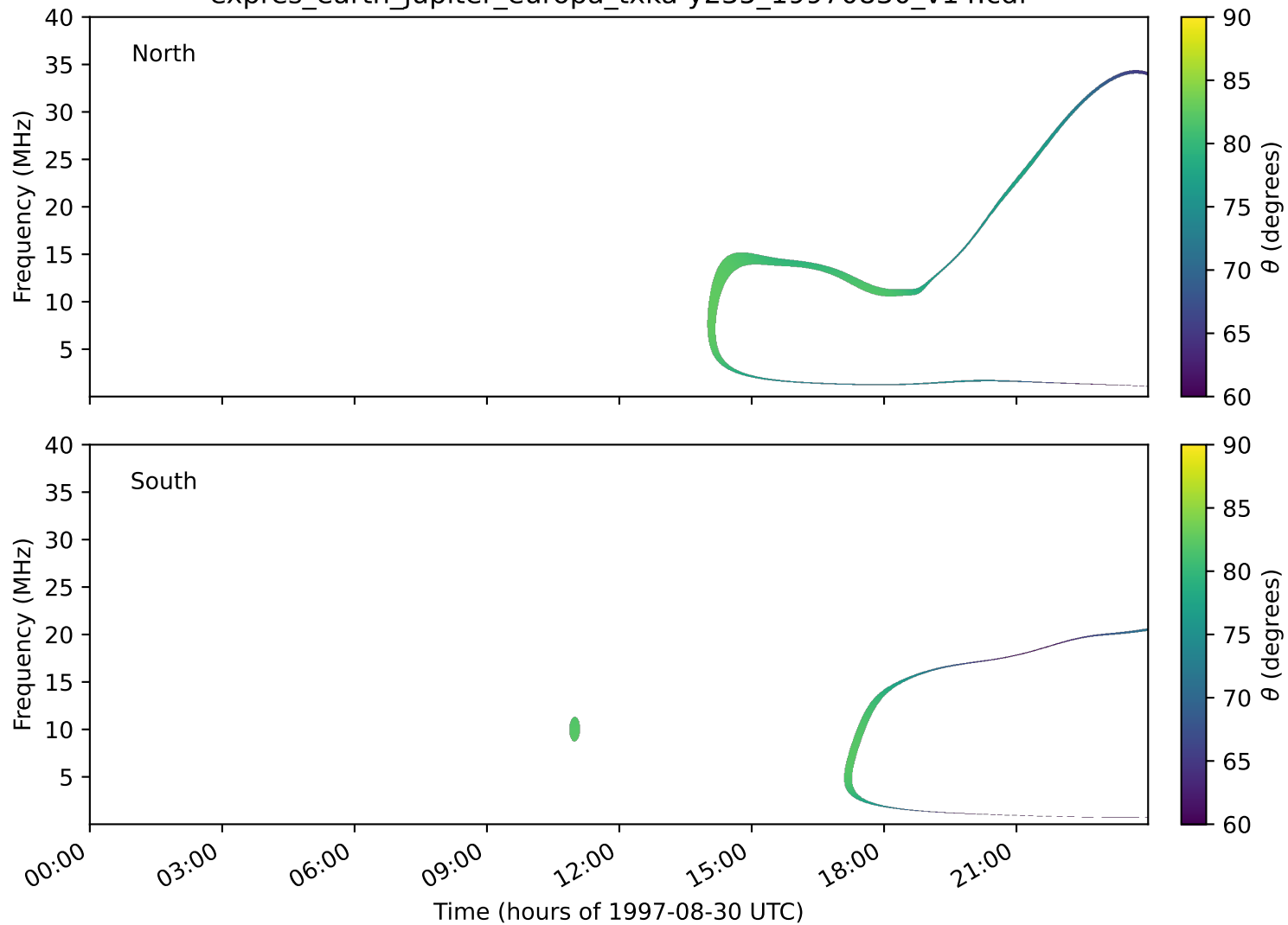
expres_earth_jupiter_europa_txka-y235_19970830_v14.cdf
