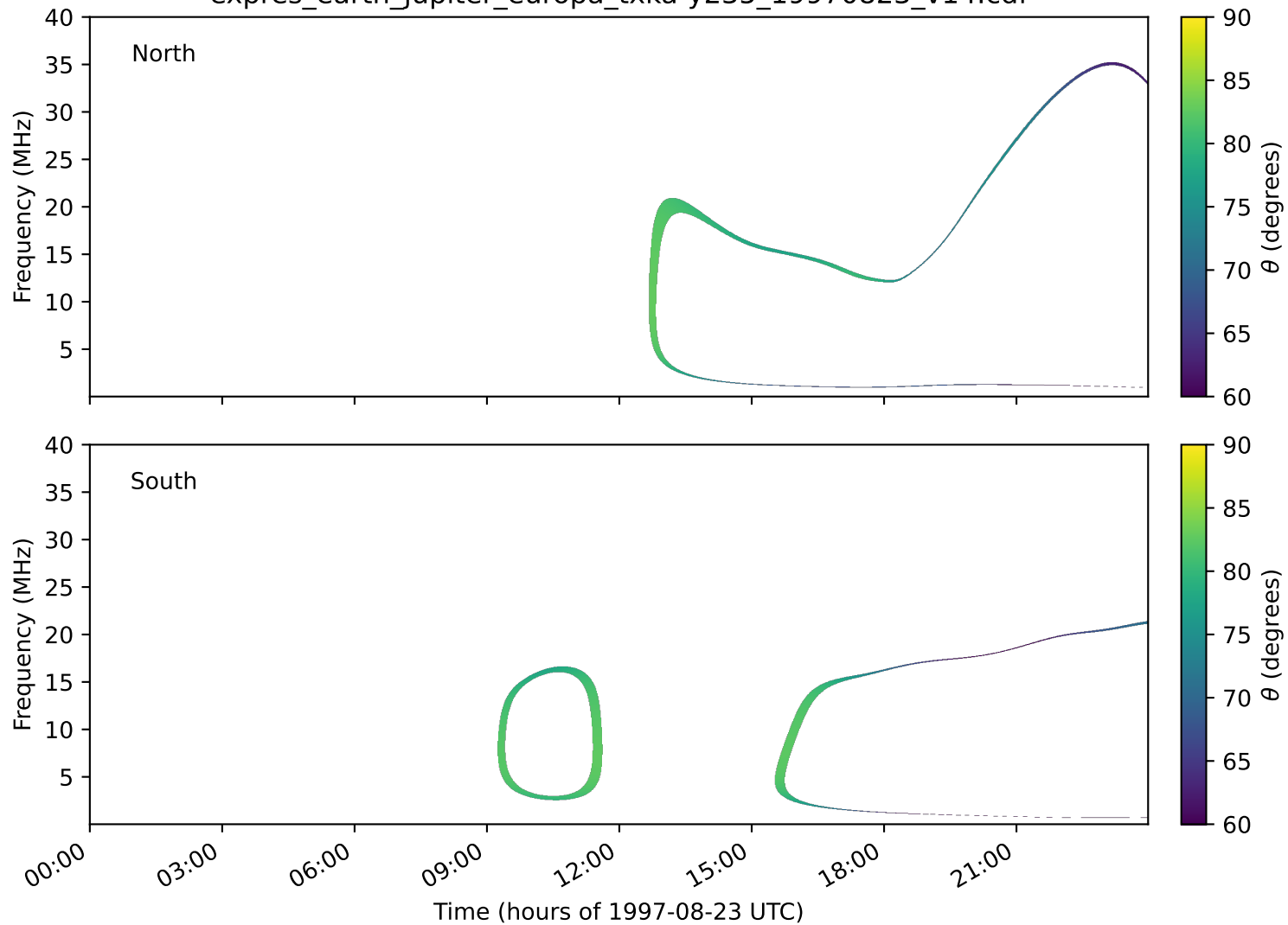
expres_earth_jupiter_europa_txka-y235_19970823_v14.cdf
