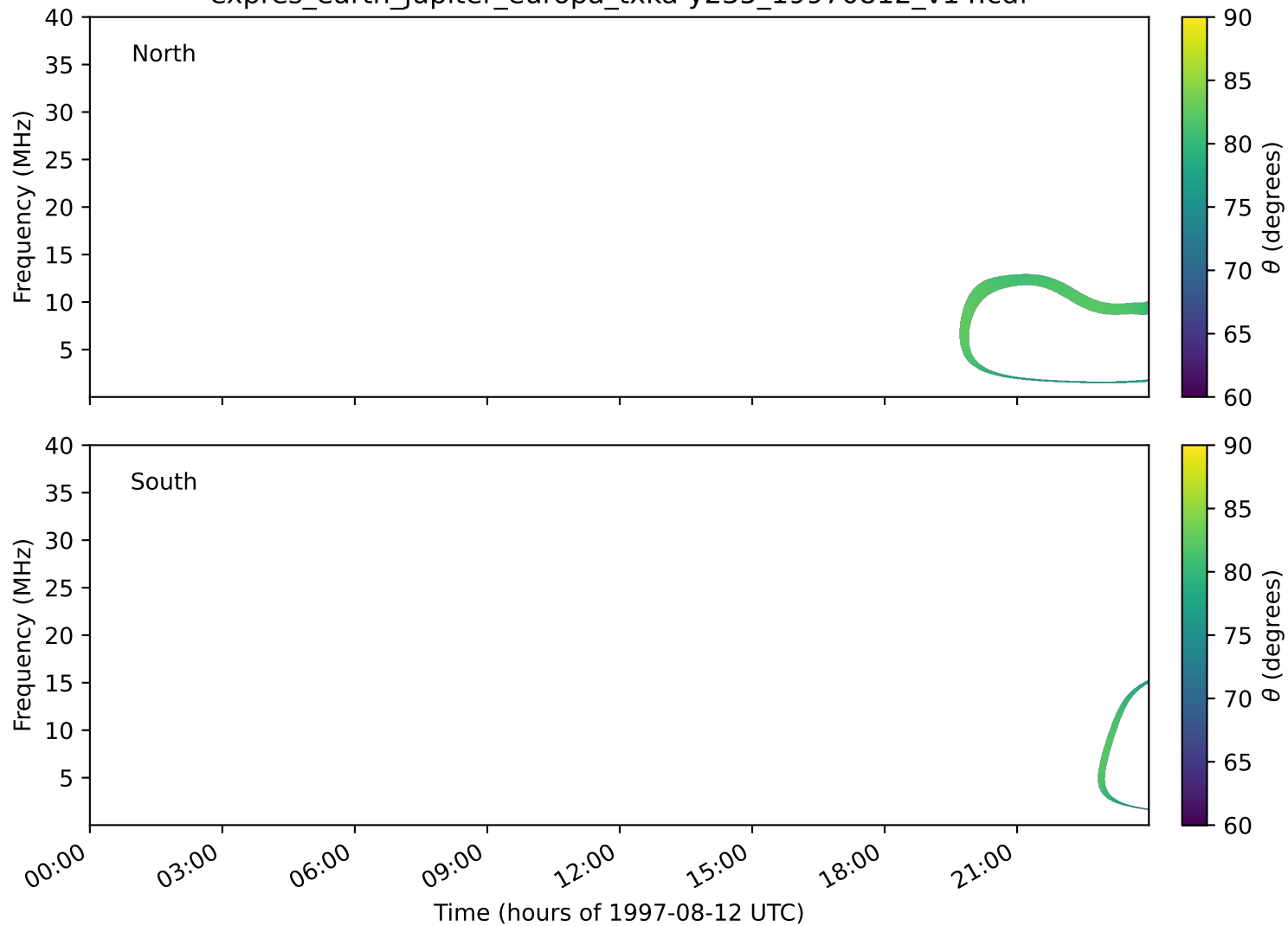
expres_earth_jupiter_europa_txka-y235_19970812_v14.cdf
